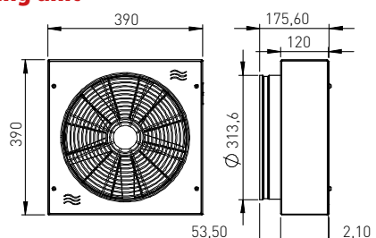
Pressurizing unit
